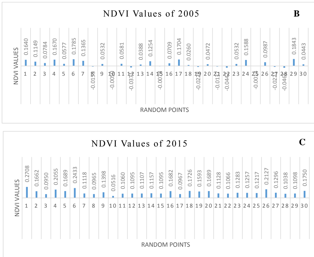
Figure:5 Random points based NDVI change detection in 1984(A), 2005(B) and in 2015(C)
