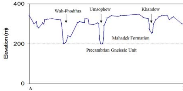
Fig.6. Topographic profile along section A-B.
