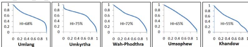
Fig. 4. Hypsometric curves of the sub-basins
