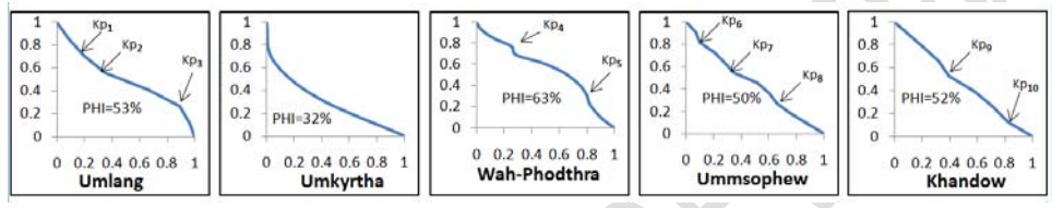
Fig. 5. Normalized longitudinal profiles
