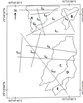
Fig.7. Diagram Map showing distribution of major lineaments
