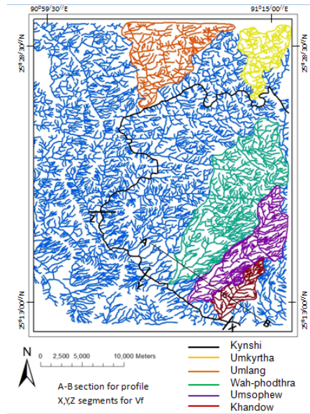
Fig. 3. Drainage map of the study area
